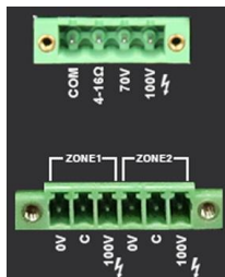
4-16Ω & 70V/100V Speaker Outputs
